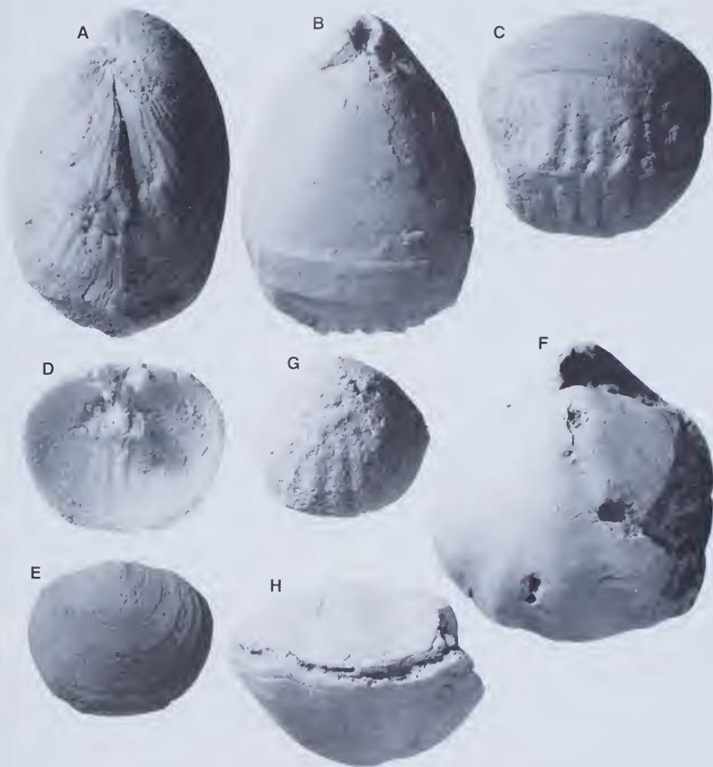
Figure 11 A–C, Indeterminate Terebratulid genus 1. A–C, WAM 88.873. A, lateral view; B, dorsal valve view; C, anterior commissure. All \times 5 . D, E, Indeterminate Terebratulid genus 2, WAM 74.1262. D, dorsal valve interior; E, dorsal valve exterior. Both \times 4 . F–H, Indeterminate Terebratulid genus 3, WAM 79.2331. F, ventral valve view \times 3 ; G, dorsal valve view \times 3 ; H, anterior commissure \times 3 .
